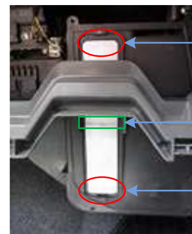
Step-15 Ensure that the "Rounded" Corners of the front plates, mate up with the upper or lower cavity surface, and that the "Flat" edges of the front plates mate up flushly with each other.
